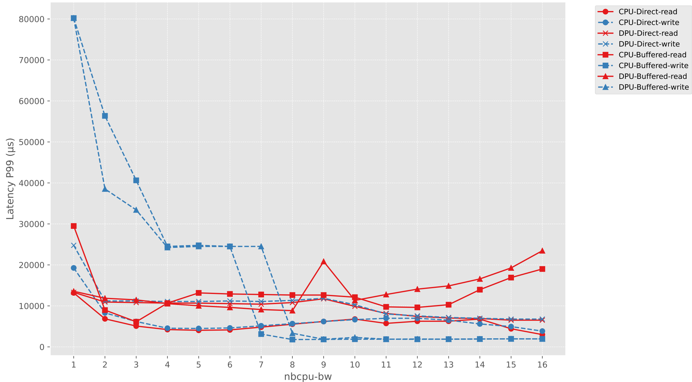
Latency P99 vs nbcpu-bw (CPU vs DPU, Direct vs Buffered)
